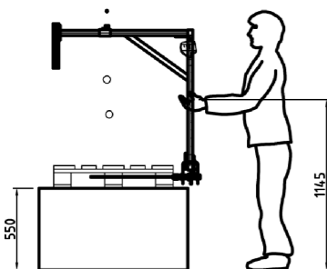
Releasing pallet
